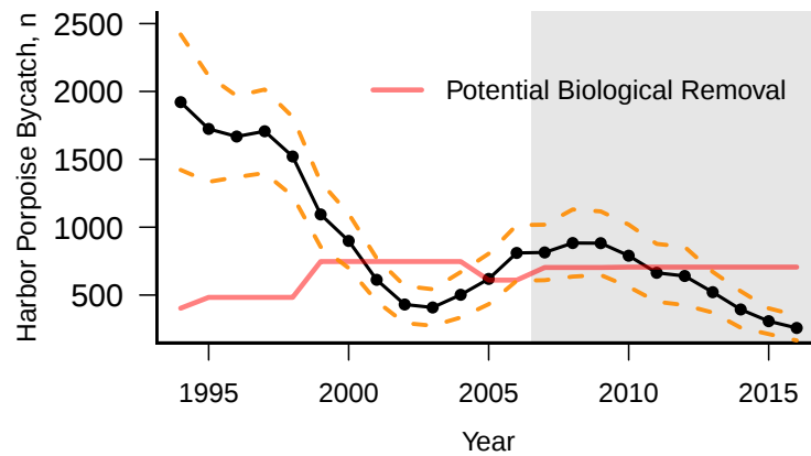
Figure 17: Harbor porpoise bycatch estimated compared with PBR
