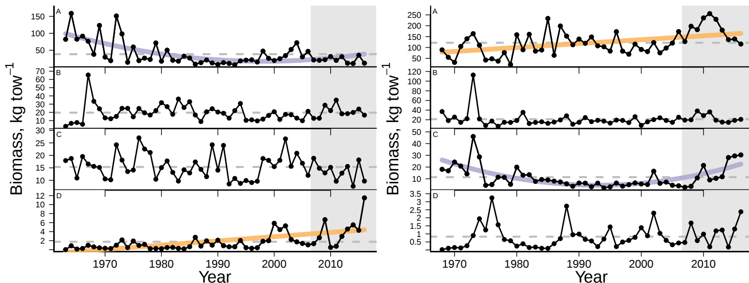
Figure 19: Fall (left) and spring (right) MAB Survey Biomass (A: Piscivore, B: Planktivore, C: Benthivore, D: Benthos)
