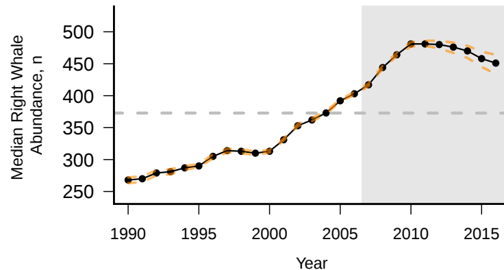
Figure 18: Right whale population estimate
