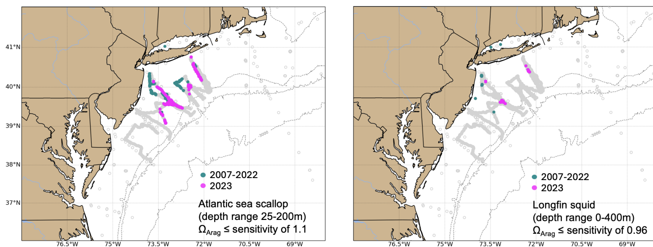
Figure 8: Locations where bottom aragonite saturation state ( \Omega_{Arag} ; summer only: June-August) were at or below the laboratory-derived sensitivity level for Atlantic sea scallop (left panel) and longfin squid (right panel) for the time periods 2007-2022 (dark cyan) and 2023 only (magenta). Gray circles indicate locations where bottom \Omega_{Arag} values were above the species specific sensitivity values.
