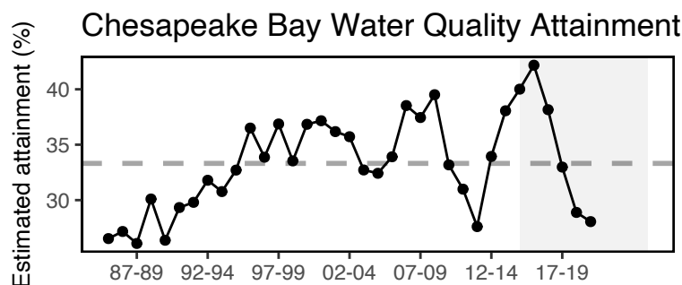
Figure 11: Chesapeake Bay water quality trend, 3 year running mean proportion of areas meeting or exceeding quality thresholds based on dissolved oxygen, chlorophyll, water clarity, and submerged aquatic vegetation.
